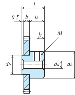
B2 type (Hub caulking)
