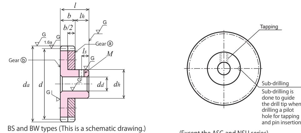
BS and BW types (This is a schematic drawing.)
