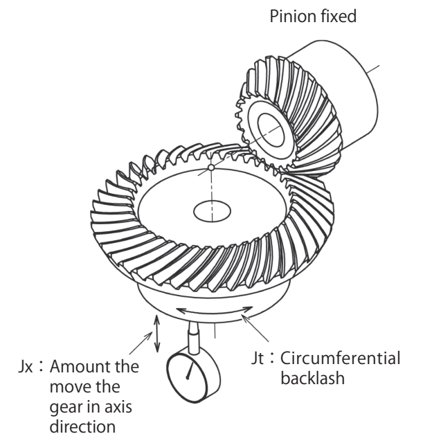
Fig.5-2 Move the pinion in axis direction to measure the backlash.
