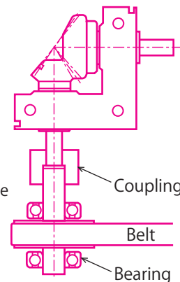
Fig. 10 Example of measure for overhang load
