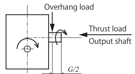
Fig. Overhang load position, thrust load, and shaft rotational direction
