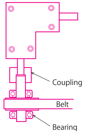
Fig. 9 Example of measure for overhang load
