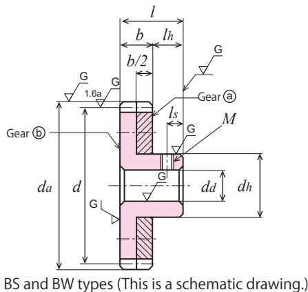
BS and BW types (This is a schematic drawing.)
