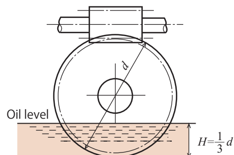
Fig. 1 Target amount of lubricating oil to be added
