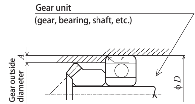
Fig. 2 Bearing housing
