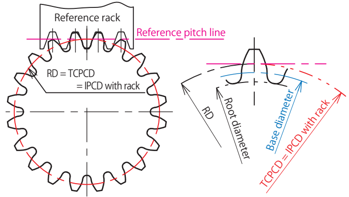
Fig. 1 Tooth profile with a rack shift coefficient ( x ) of 0
