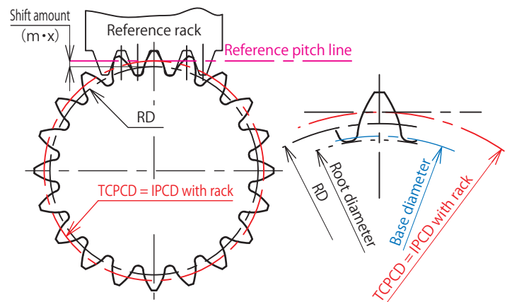
Fig. 2 Tooth profile with a positive (+) rack shift coefficient ( x )
