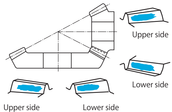
Fig.6-7 Ideal tooth bearing for Bevel gear
