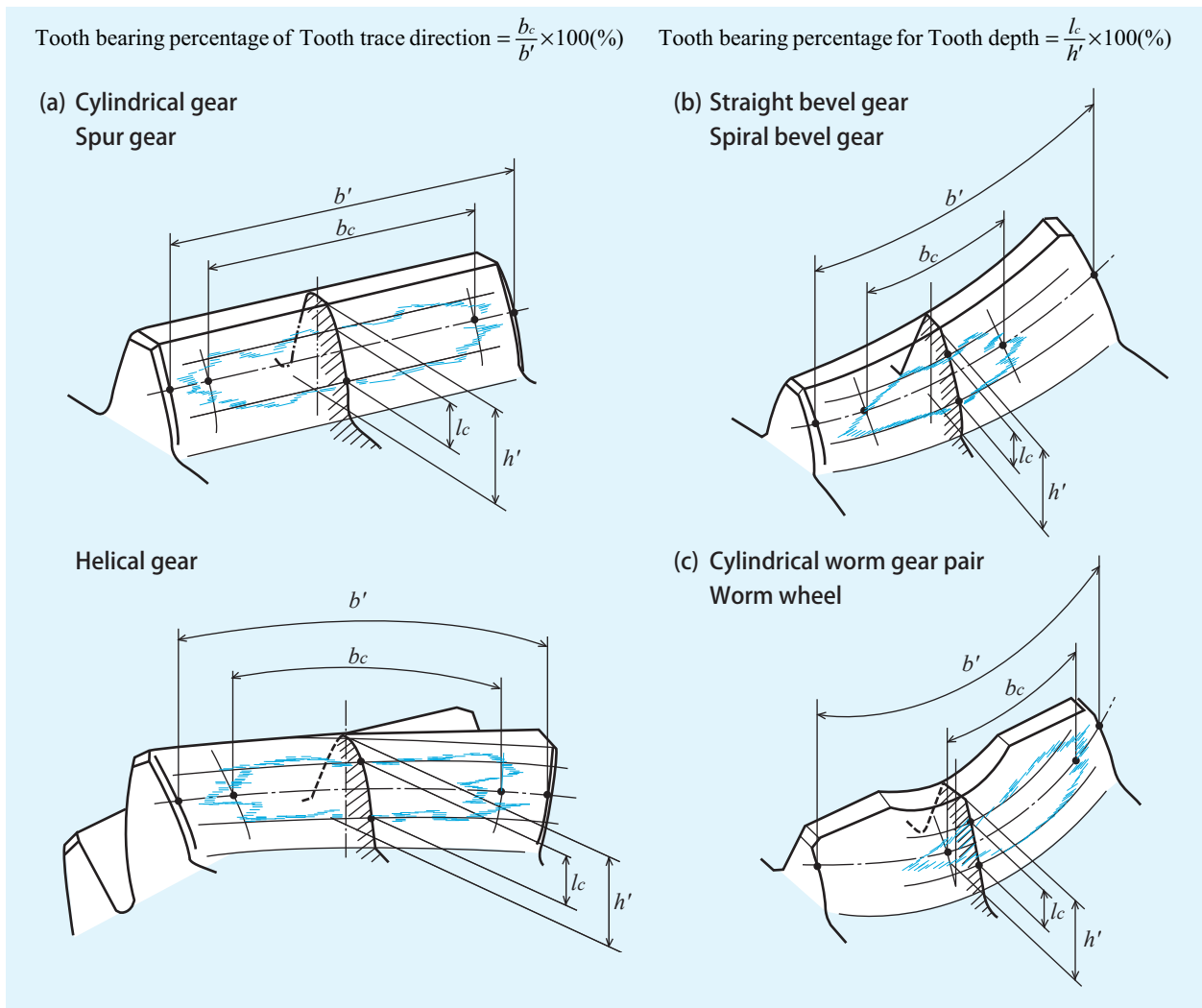
Fig. 6-1 Tooth bearing
