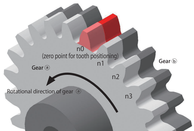
Fig. 2 Zero point for tooth positioning (n0)
